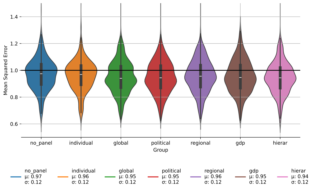
Figure 16: Forecasting: panel structure performance
