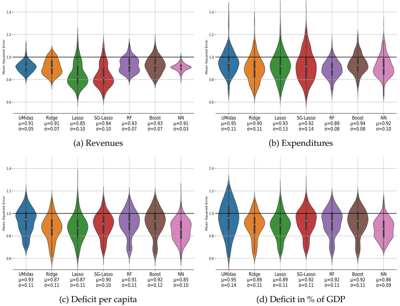
Figure 4: Models' performance by variable
