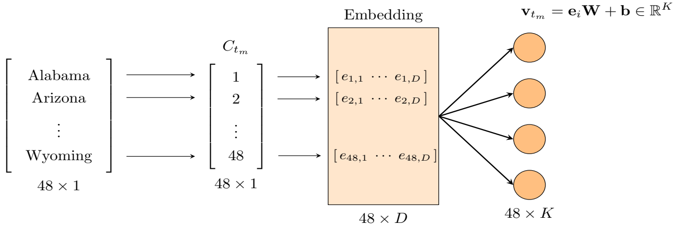
Figure 13: Embedding Layer
