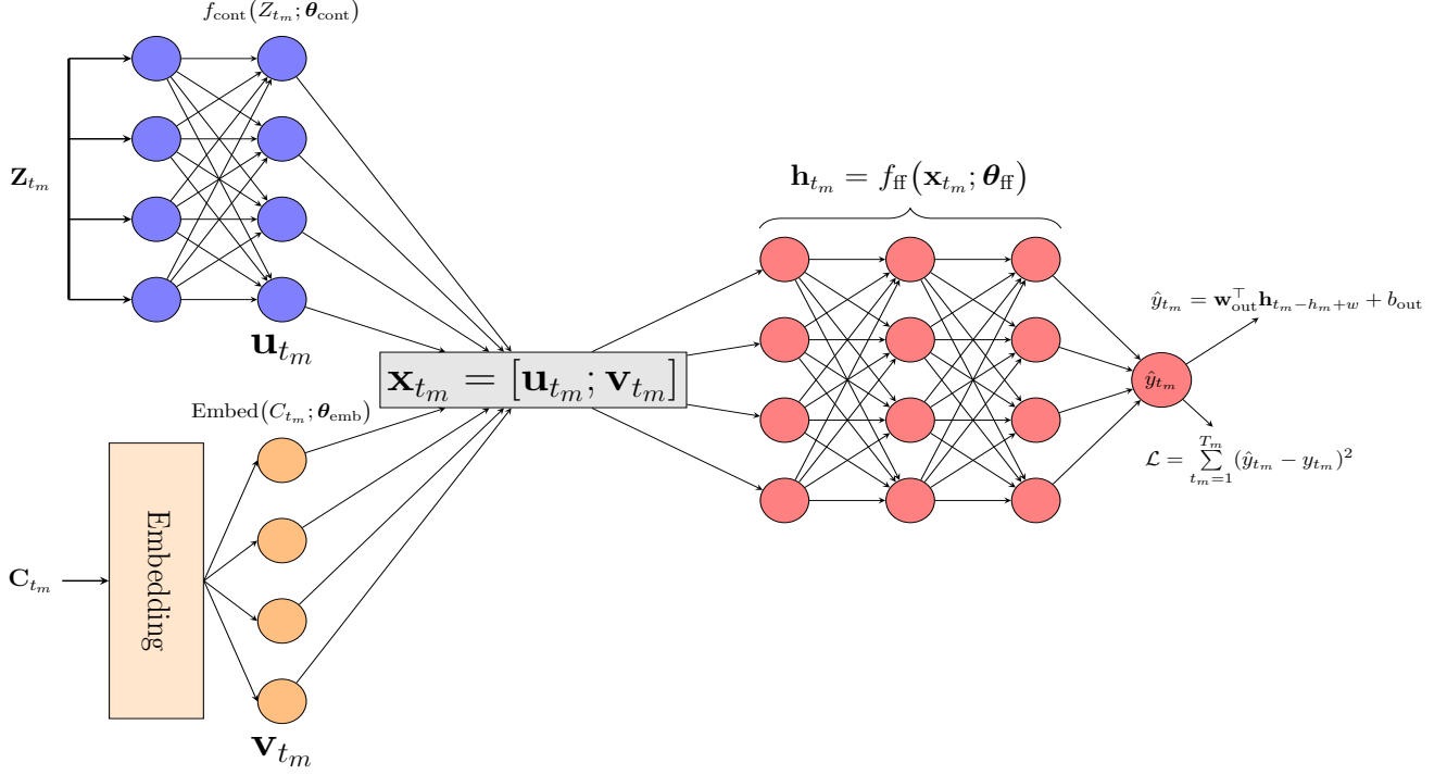
Figure 1: Neural network architecture
