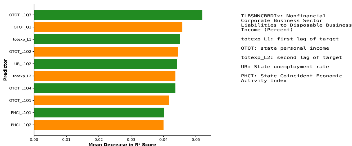
Figure 10: Nowcasting total expenditures: selected predictors
