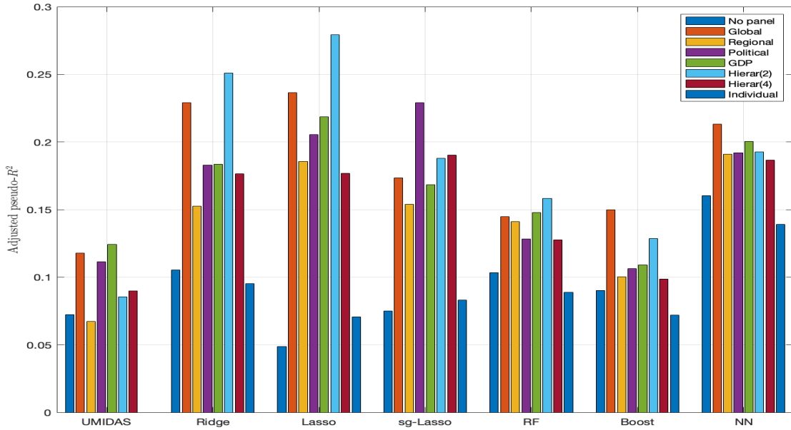
Figure 12: Pseudo- R^2 by model and panel structure
