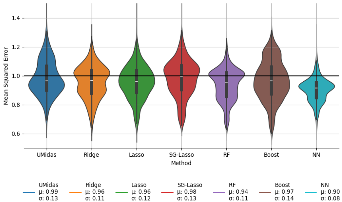
Figure 15: Forecasting: models' performance
