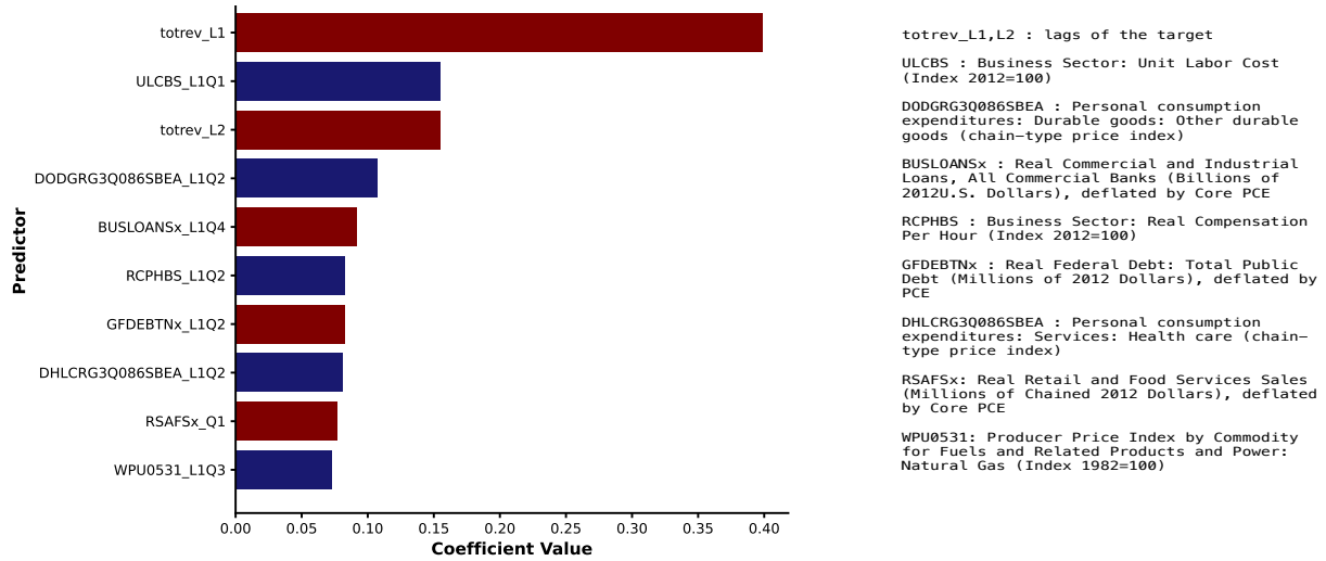
Figure 8: Nowcasting total revenue: selected predictors
