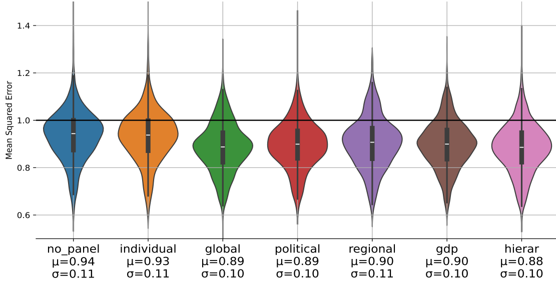
Figure 5: Average impact of clustering
